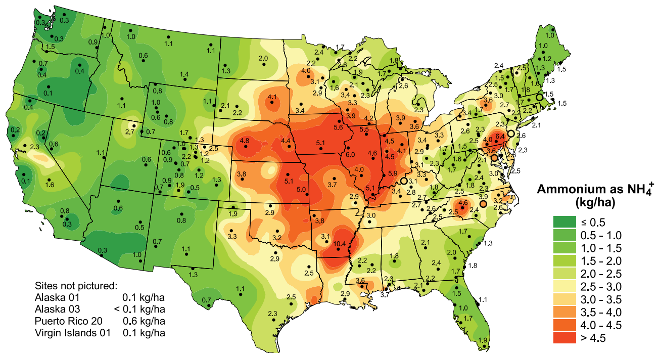
Ammonium ion concentration (top) and wet deposition (bottom), 2009.
